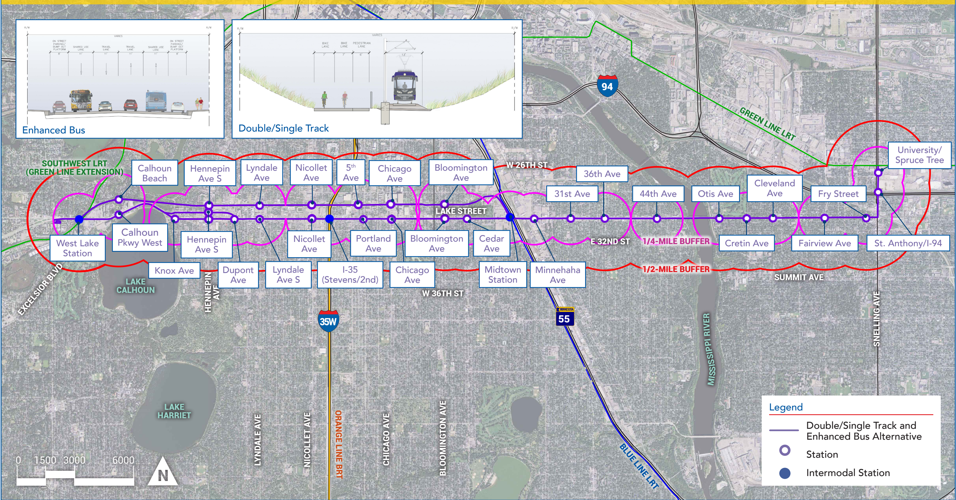
Figure 3. Dual Alternative – Double/Single Track (Greenway) and Enhanced Bus (Lake Street)
