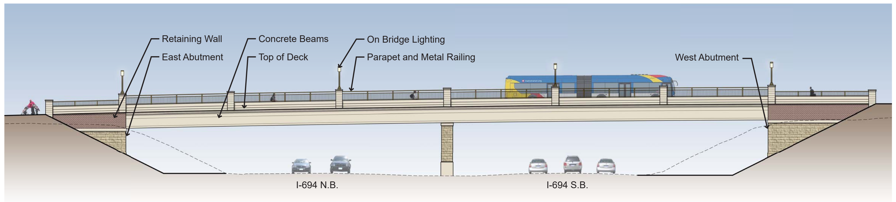
Elevation of Pedestrian Facility Treatment
