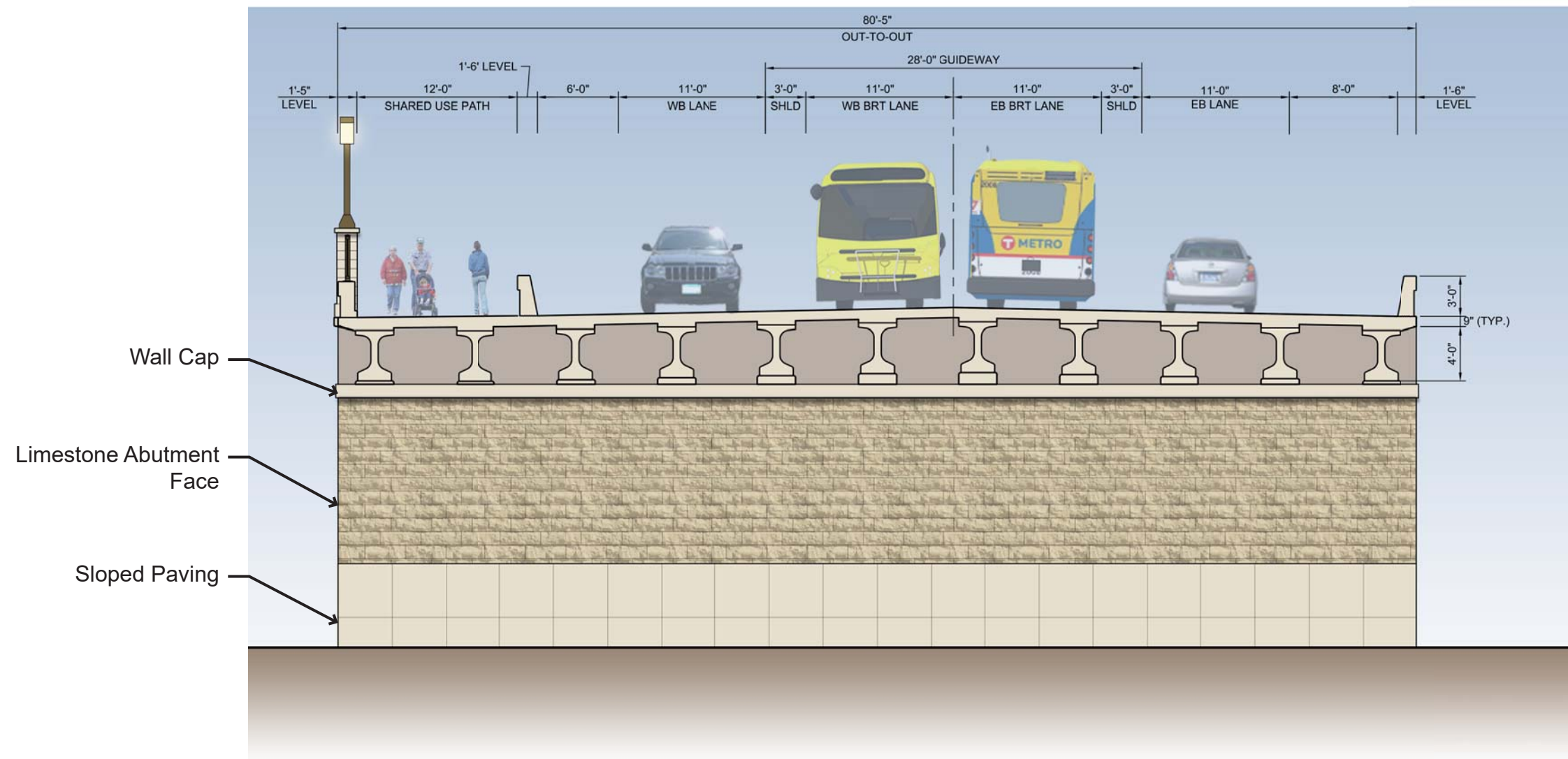
East Abutment
