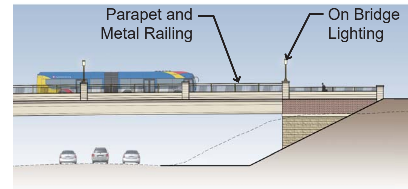
Elevation of Pedestrian Facility Treatment
