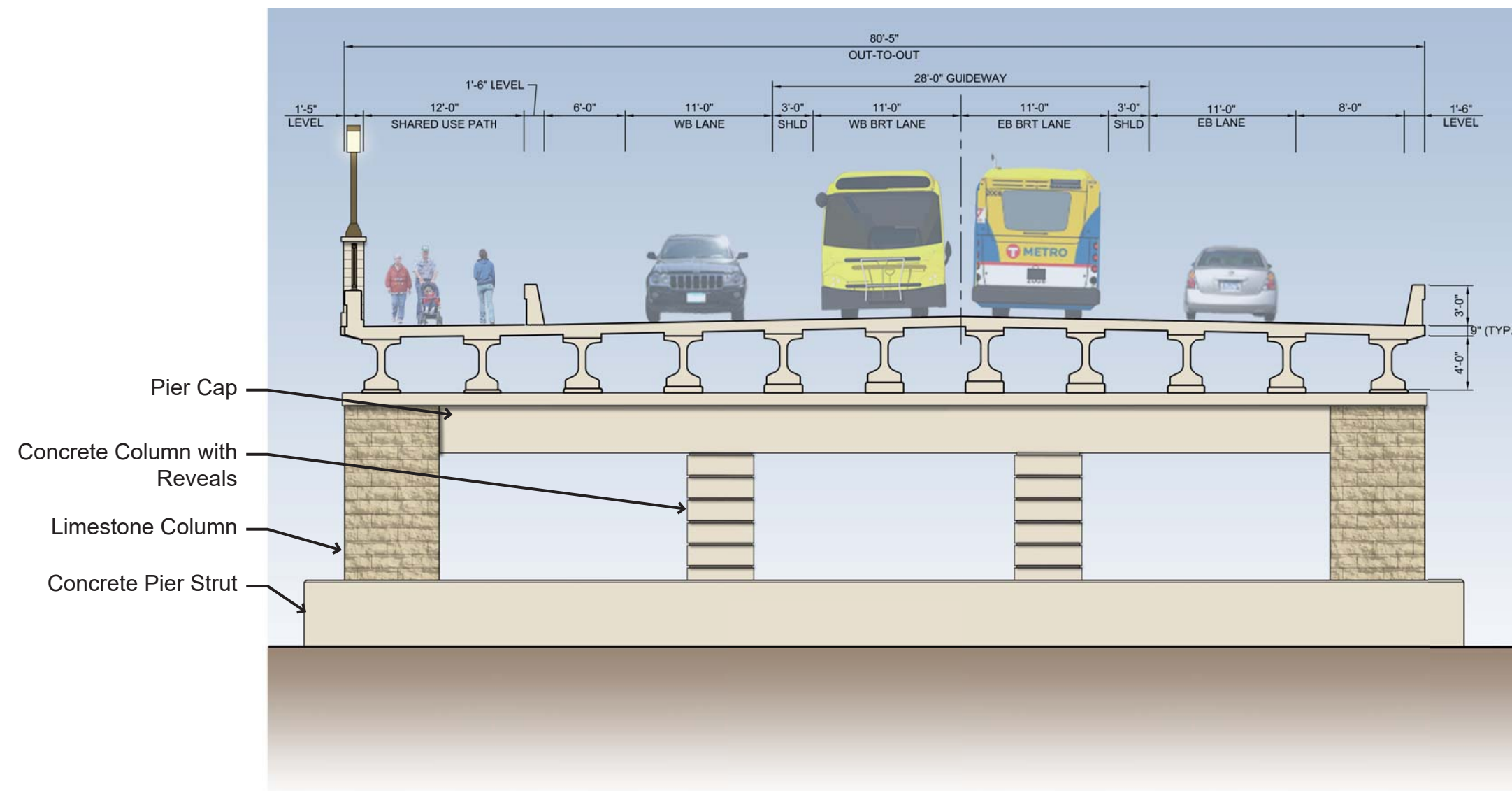
Pier Elevation Looking East
