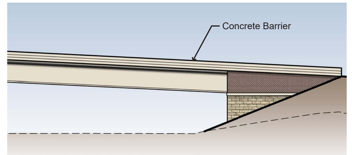
Elevation of Roadway Treatment
