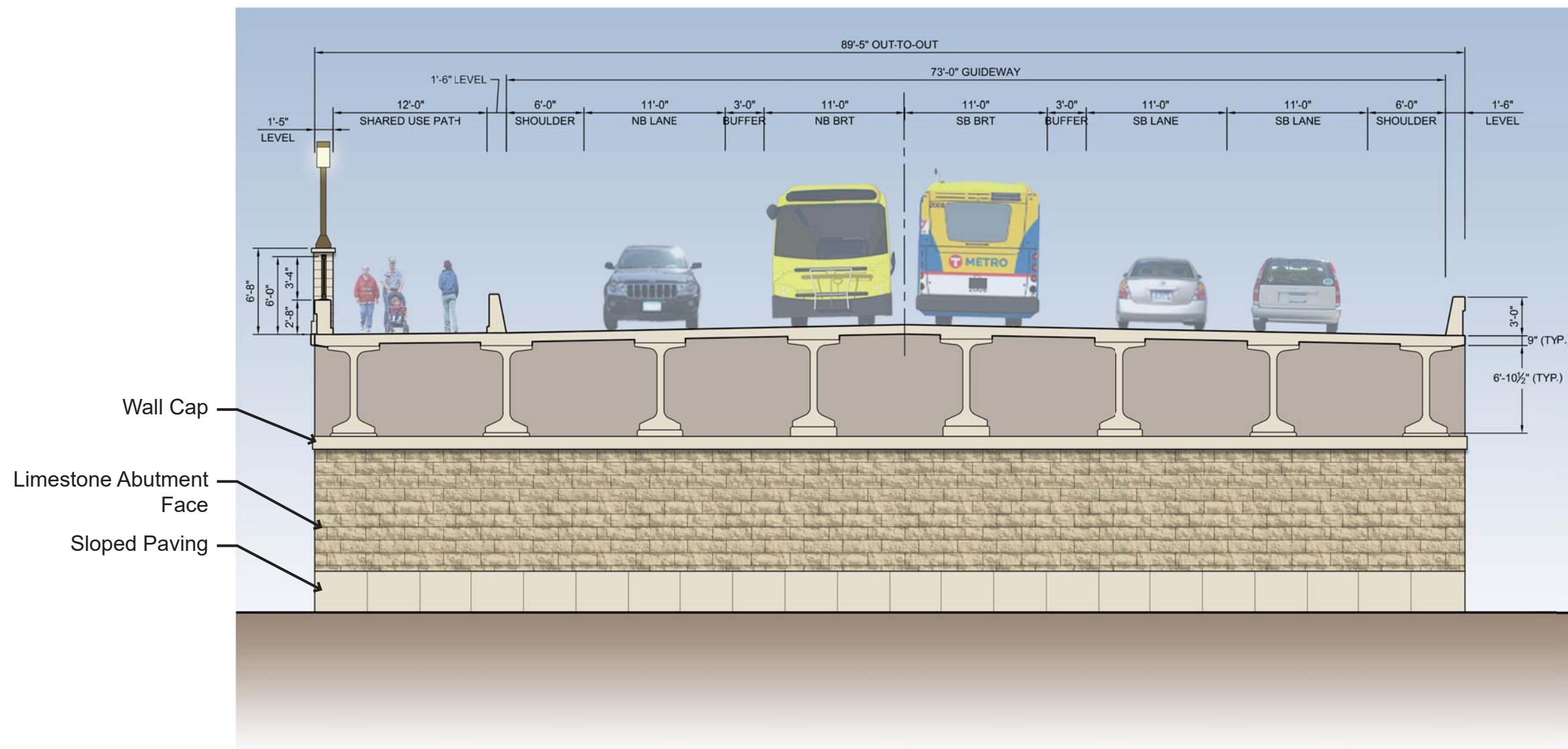
South Abutment
