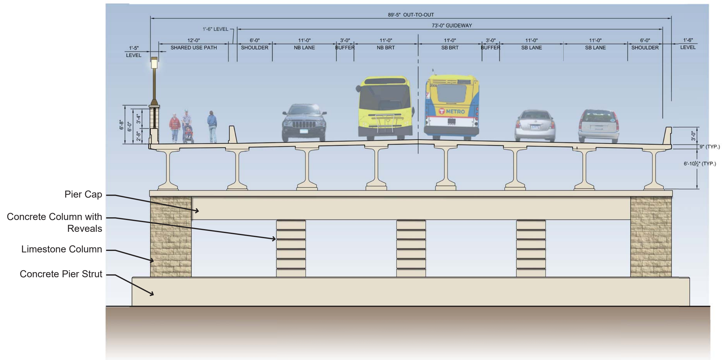
Pier 2 Elevation Looking South
