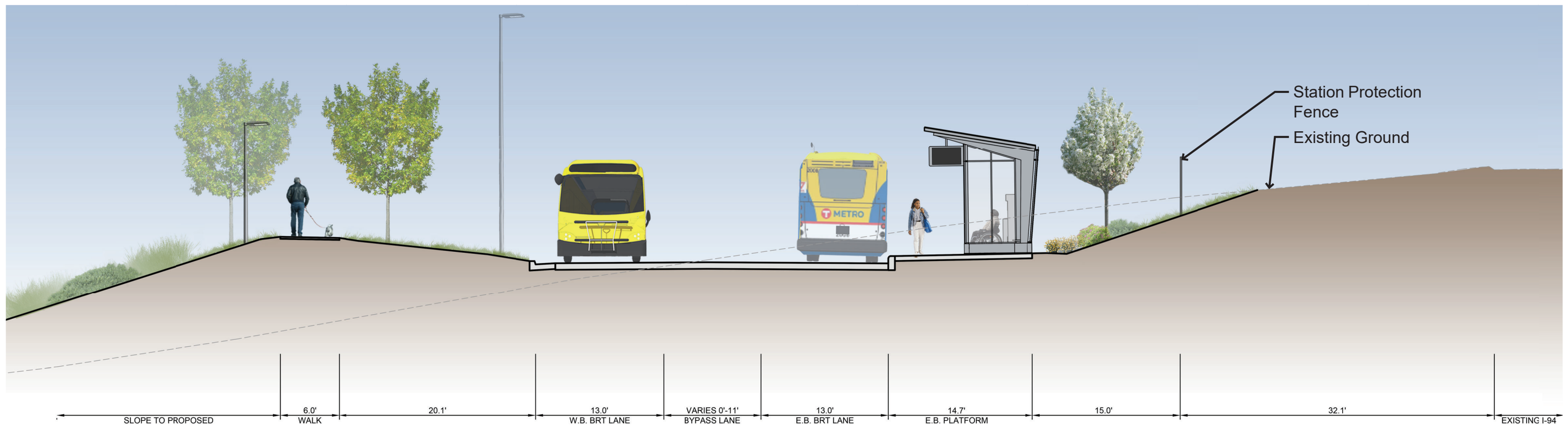
Section B-B: E.B. Platform (Looking East)
